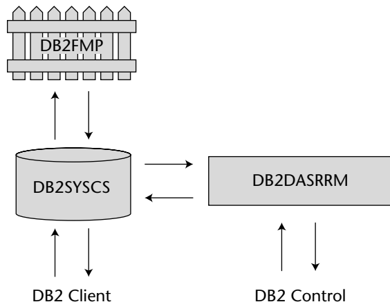
Figure 6-1 DB2 processes.
