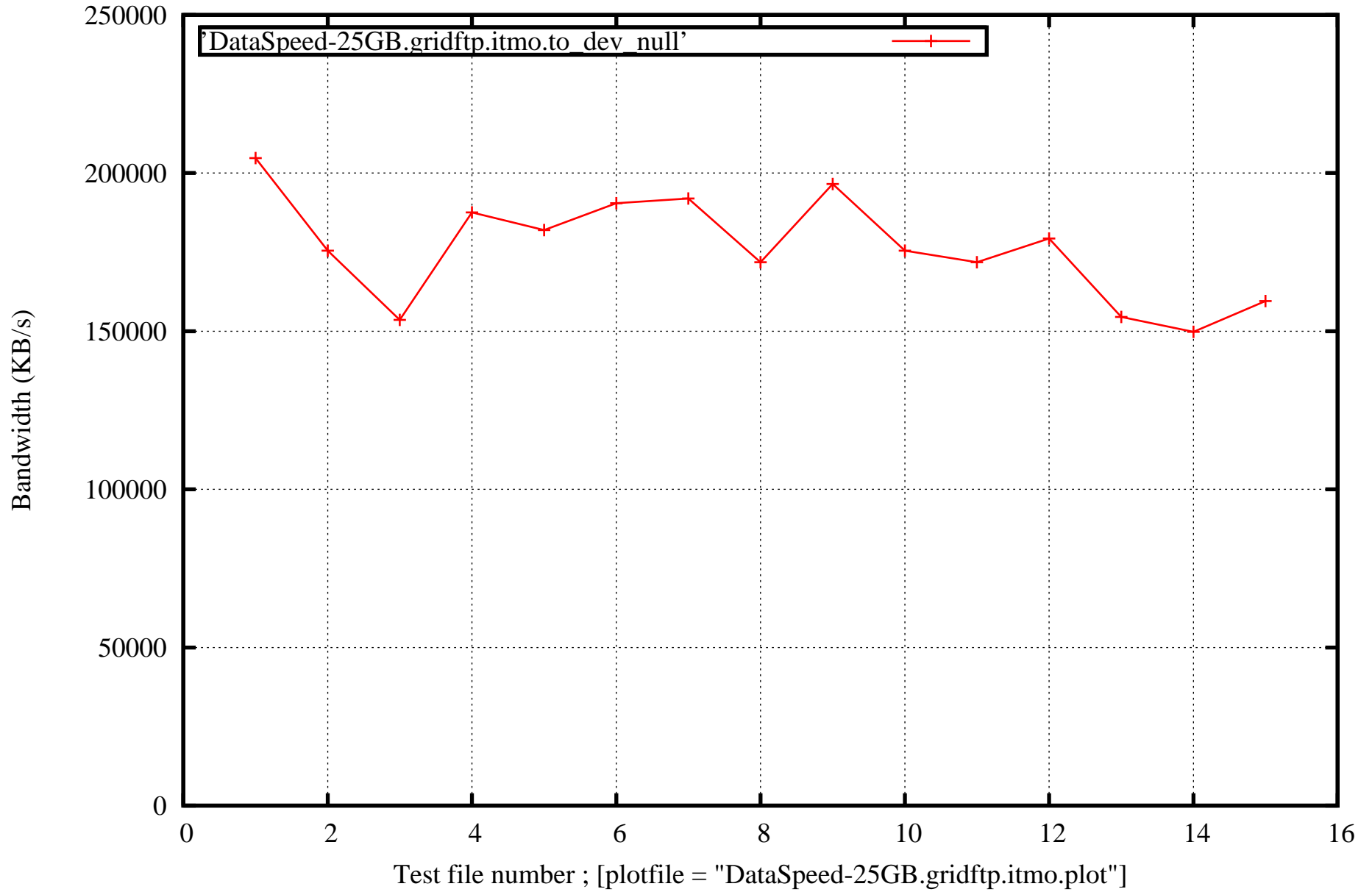
Data Transfer Speed. Data Size 25 GB. GridFTP
