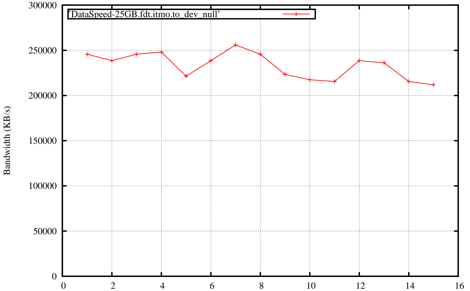
Data Transfer Speed. Data Size 25 GB. FDT
