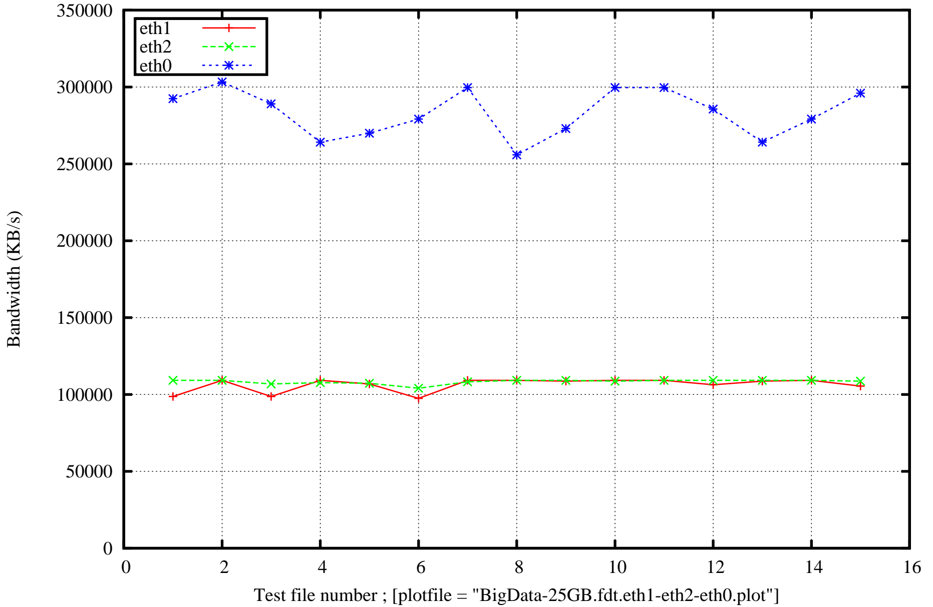
Data Transfer Speed. Data Size 25 GB. FDT. eth1 eth2 eth0
